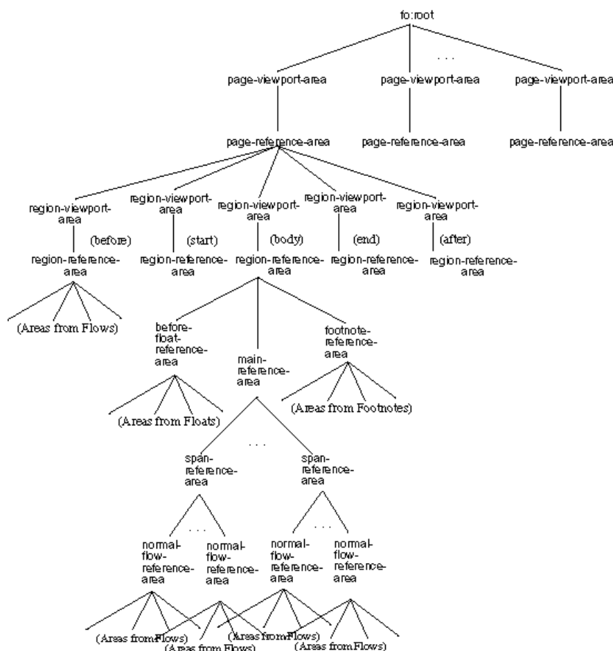
A Typical Area Tree
