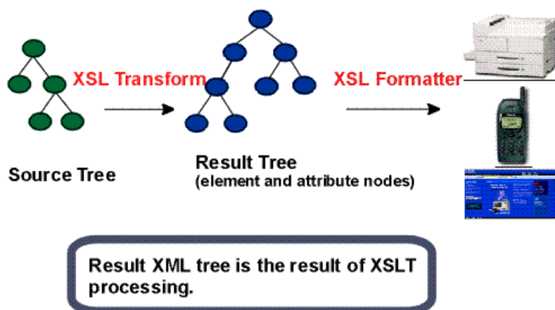
XSL Two Processes: Transformation &amp; Formatting
