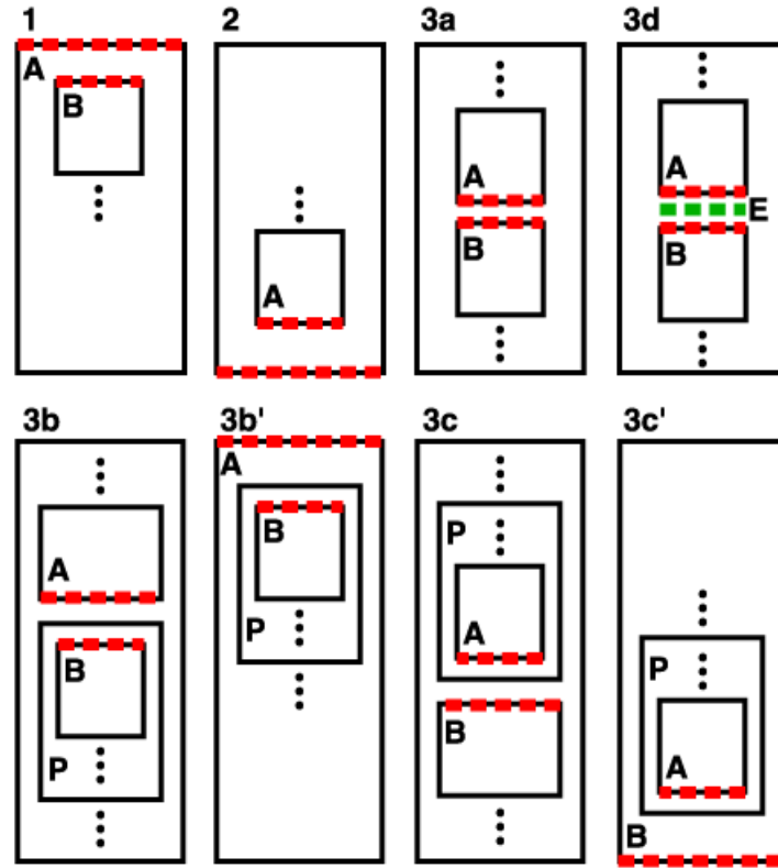
Adjacent Edges with Block-stacking
