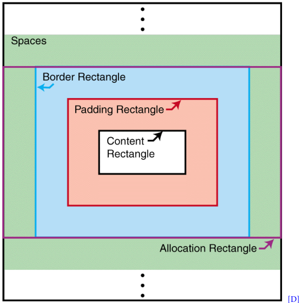
Allocation- and content-rectangles of a block-area
